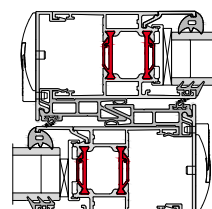
BSC94 Dual Rail/ Tri Rail – Standard Interlock
