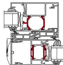
BSC94 Mono Rail – Interlock
