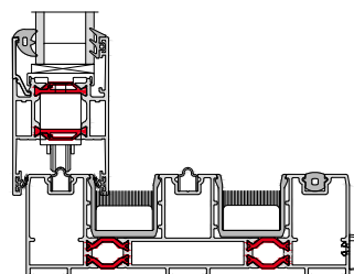
BSC94 Dual Rail/Tri Rail – Standard Slimline Interlock
