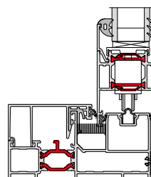
BSC94 Mono Rail – Cill
