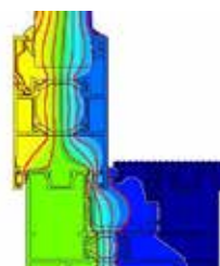
BSC94 Thermal Profile
