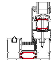
BSC94 Dual Rail – Cill
