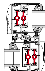
BSC94 Dual Rail/Tri Rail – Standard Slimline Interlock
